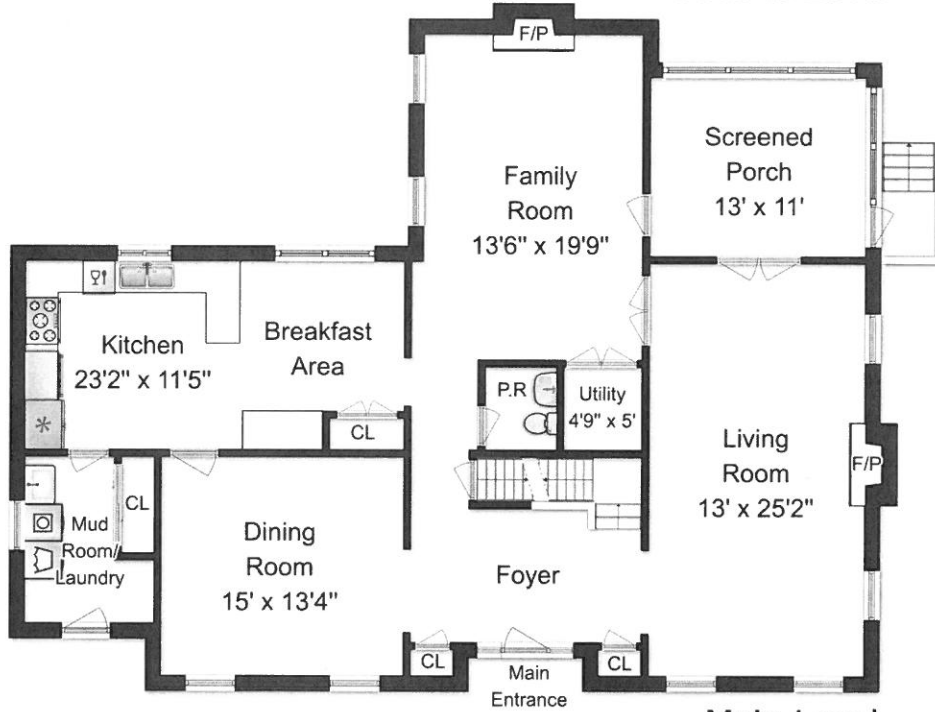
Main Level
